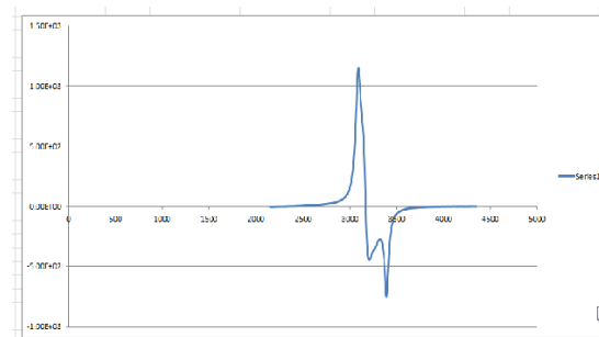
Fig (11): The curve for complex Cu-cell
