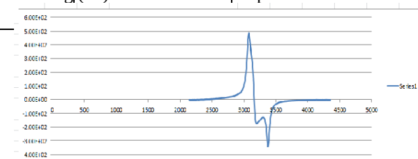
Fig (13): The curve For complex Cu-copolymer
